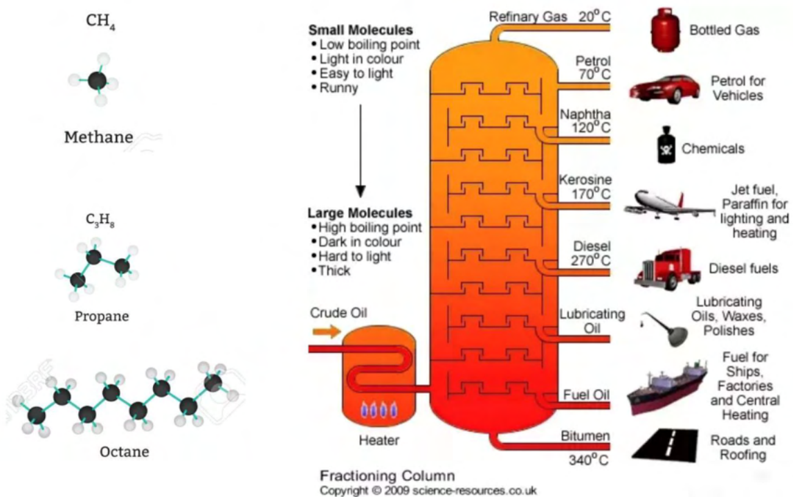
Fractional Distillation of Crude Oil
