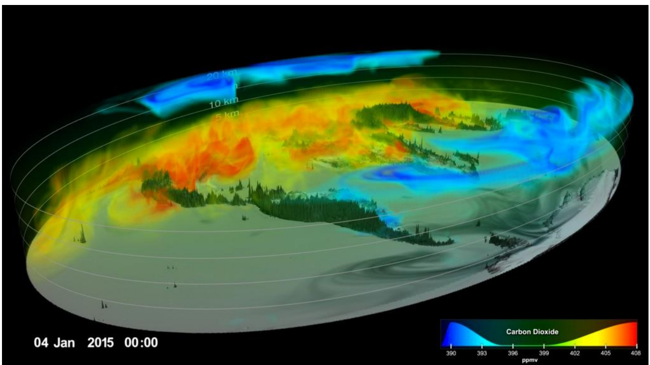
NASA, 3D Simulation, Carbon Dioxide (CO2), Goddard Space Flight Center, Greenhouse Gas, OCO-2, Jet Propulsion Laboratory, Global
