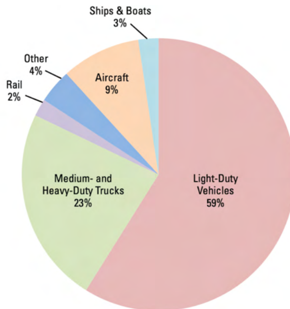
U.S. Transportation Sector GHG Emissions by Source, 2017
